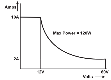
Autorangeing Curve for 60 V/10 A/120 W Power Module
